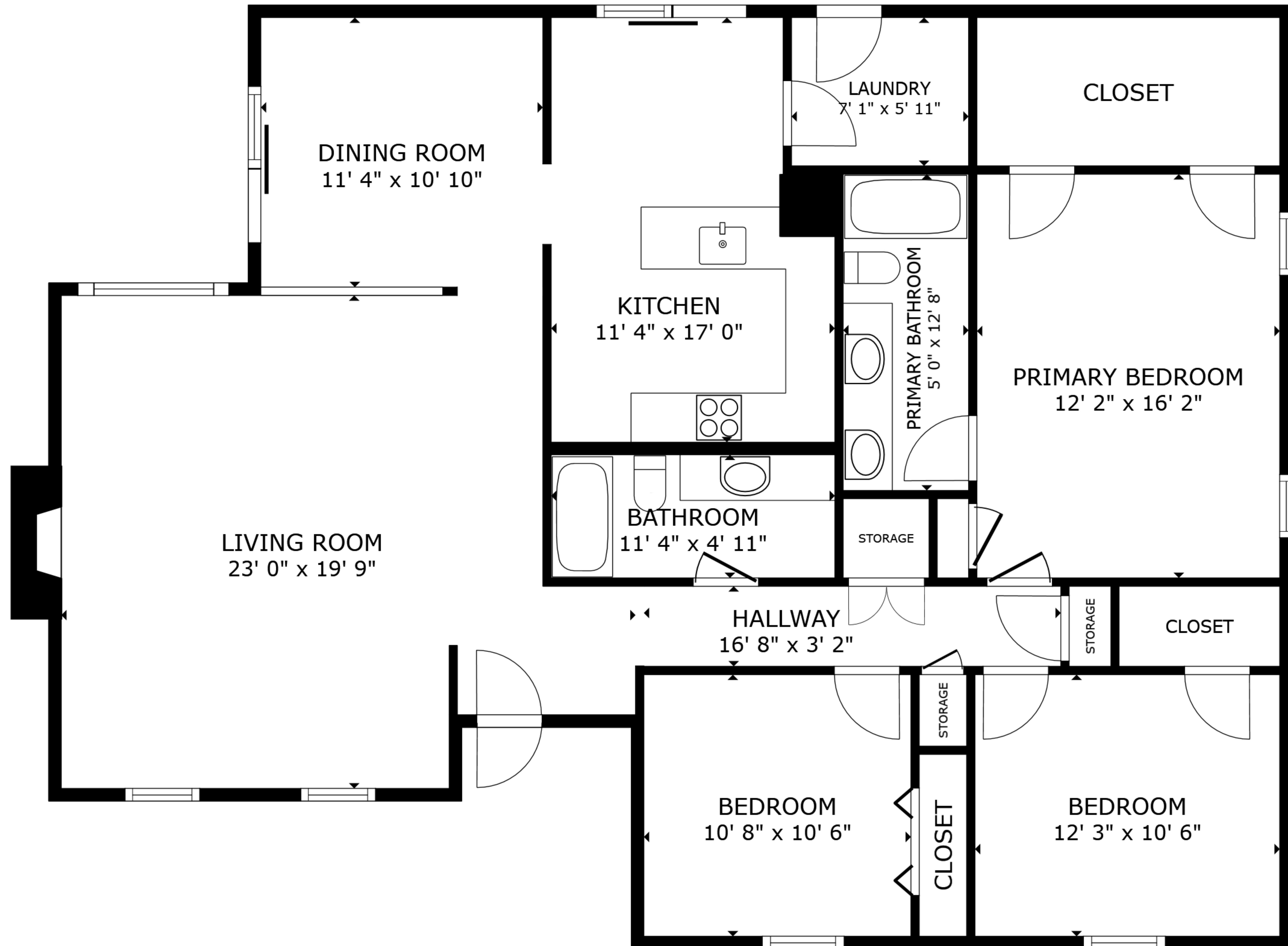
FLOOR PLAN
